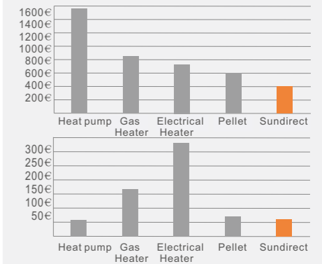
The above chart roughly compares equipment costs between all kinds of heaters on the market. The bottom chart compares the operating costs between all kinds of heaters. The calculation assumes 15m 2 room size (standard in Europe), the number is subject to change in different countries.
